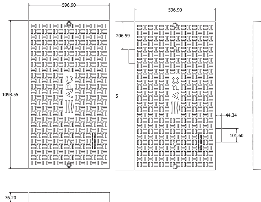
LOCKING DETAIL (BOLTS ON TO TROUGH)
